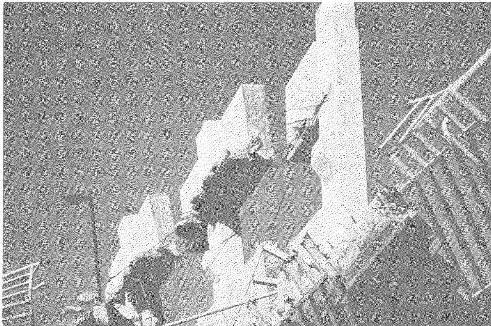
Fig. 52 CSUN parking structure. Note brackets for supporting precast girders and minimal continuity reinforcement.
