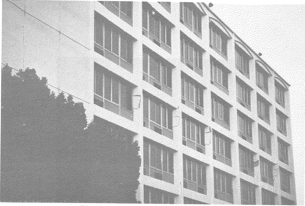
Fig. 49 Diagonal cracking of frame columns.
