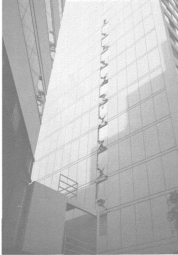
Fig. 46 Diagonal tension failure of coupling beams.
