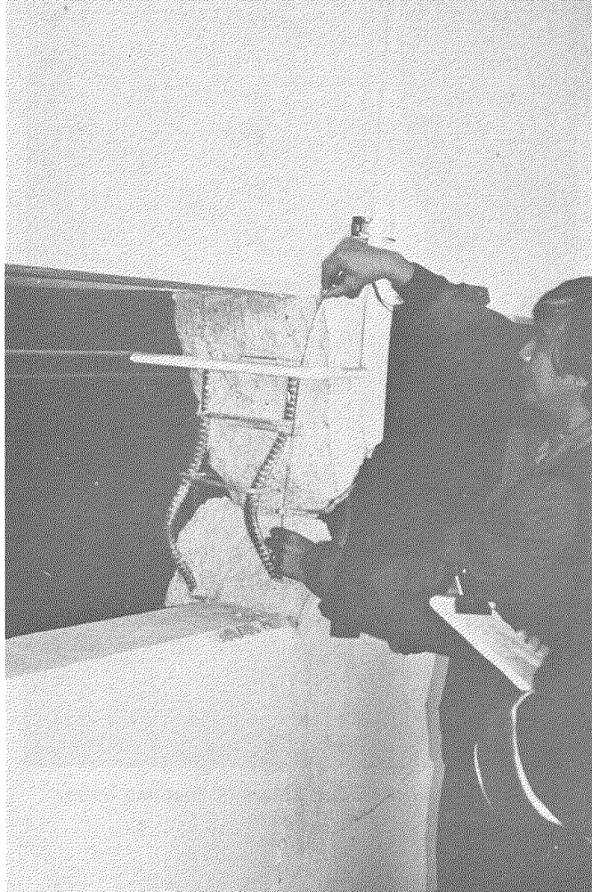
Fig .47 Short column shear failure.
