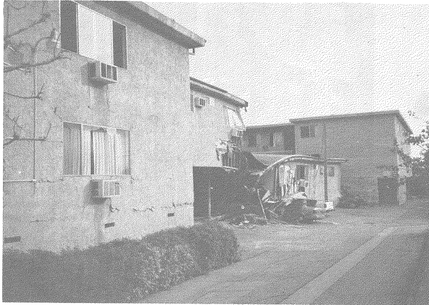
Fig. 39 First soft-story collapse of a timber structure.
