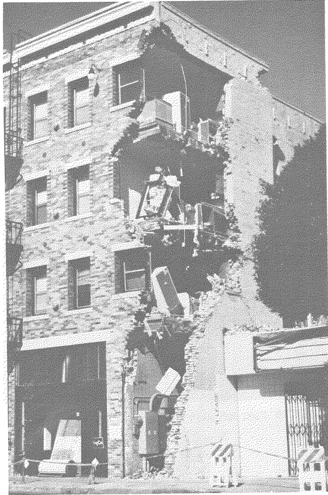
Fig. 40 Masonry crushing and out-of-plane failure.
