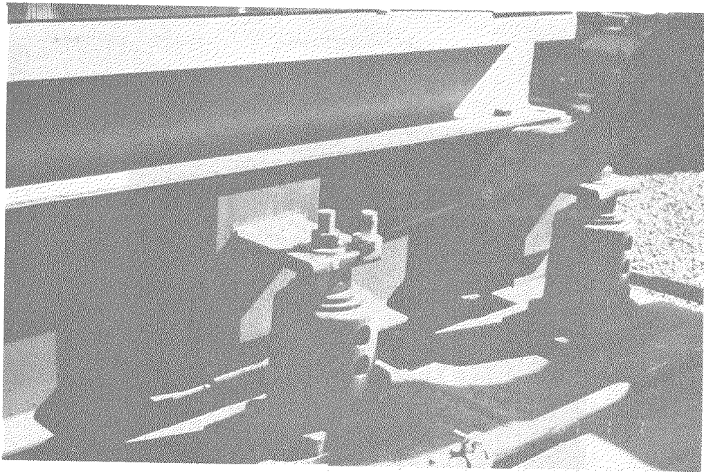
Fig. 36 The base plate of a steel structure allowed relative movements between slab and steel structure.
