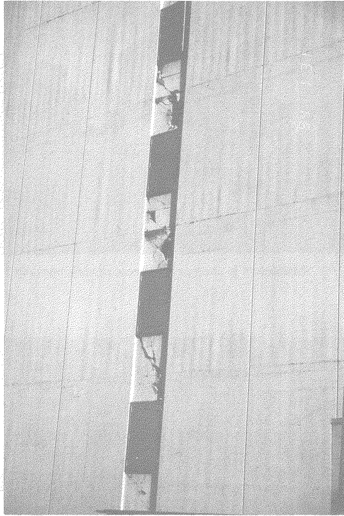
Fig. 31 Detail of shear damage in coupling beams.
