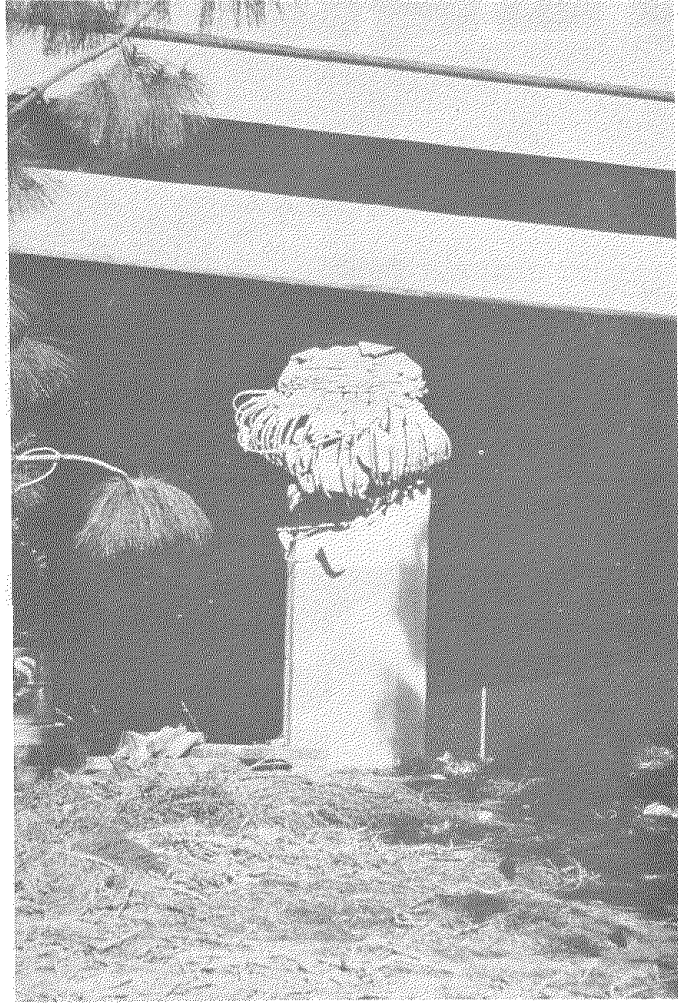
Fig. 28 Column flexural hinging.
