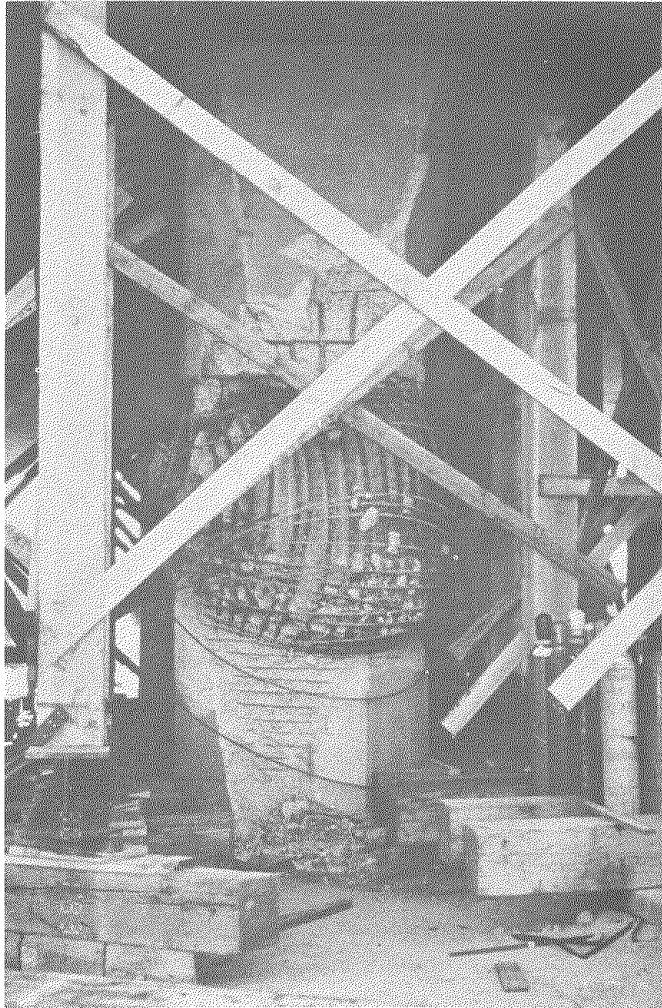
Fig. 27 Shear compression failure and rebar buckling in bridge columns.
