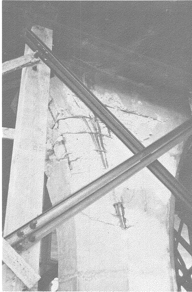
Fig. 26 Shear compression failure and rebar buckling in bridge columns.
