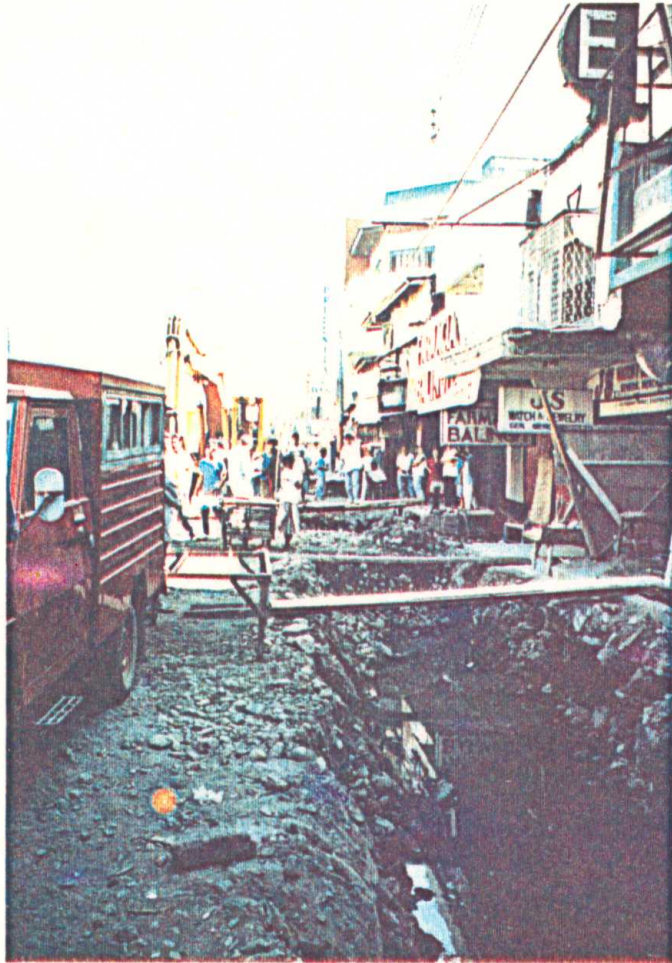
Photo 4.22 Reconstruction of the main sewage line in Hernandez Avenue of Dagupan City. High level of ground water table.
