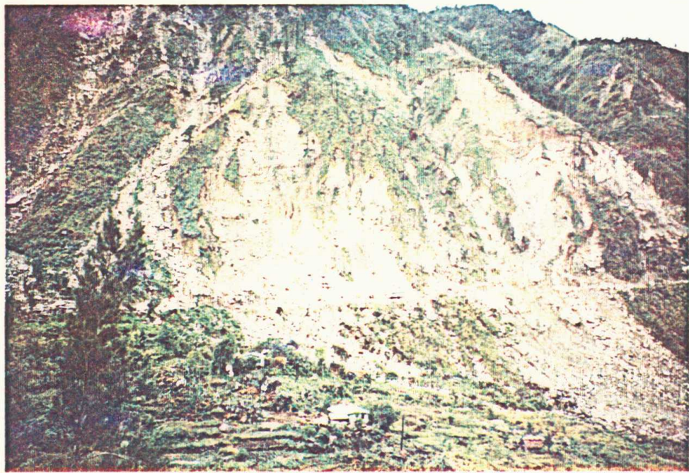
Photos 3.20 Intensive medium scale rockfall on the Marcos Highway approaching Baguio City.
